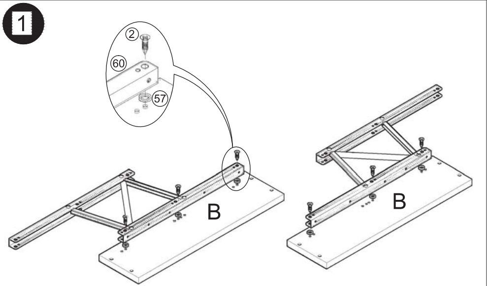
MESA ELEVABLE 100x50 cm
